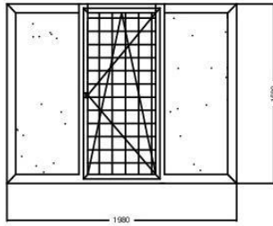
Ferestre parter; 1980x1580(h) -14 buc
