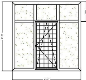
1. Ferestre; 1760-x2100(h) -4 buc
