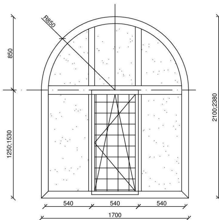
1. Ferestre parter, etajul N1; 1700-x2100;2380(h)
