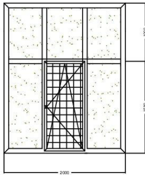
1. Ferestre; 2000-x2580(h) -13 buc
