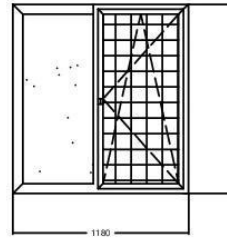
Ferestre; 1180-x1580(h) -68buc Ferestre; 1160-x1580(h) -36buc
