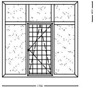
1. Ferestre parter, etajul N1; 1700-x2200(h) -24 buc
