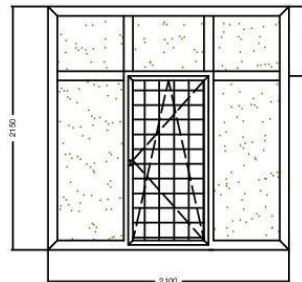
1. Ferestre; 2100-x2150(h) -1buc
