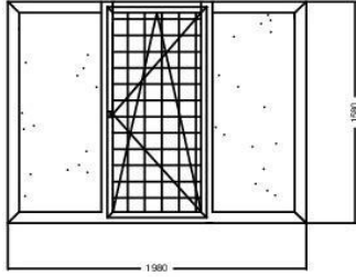
Ferestre parter; 1980x1580(h) -9 buc
