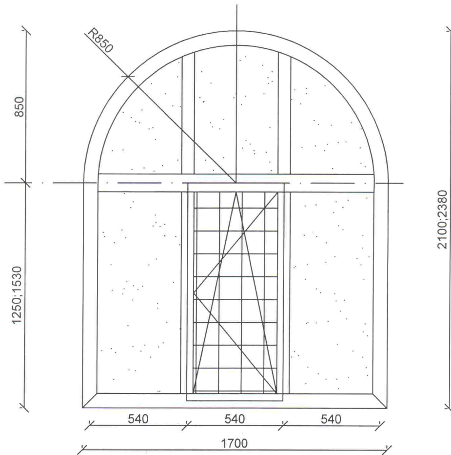
1. Ferestre parter, etajul N1; 1700-x2100;2380(h) -53 buc
