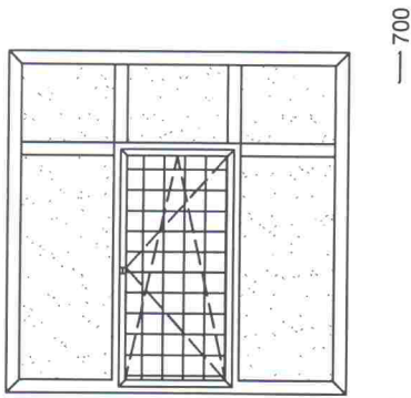
1. Ferestre parter,etajul N1; 1700-x2280(h) -32buc
