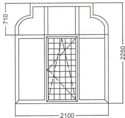
1. Ferestre; 2100-x2250(h) -1 buc
