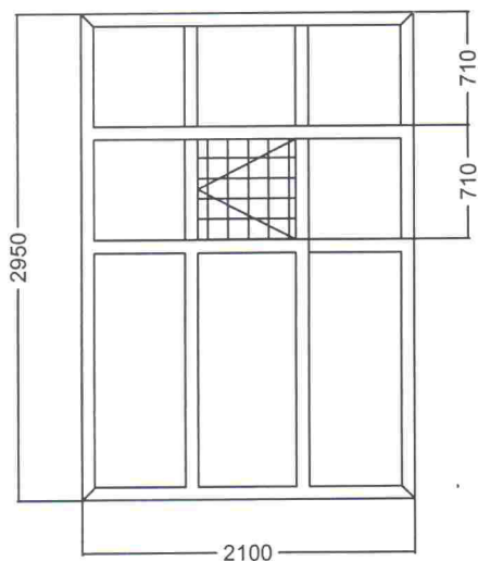
1. Ferestre; 2100-x2950(h) -1 buc
