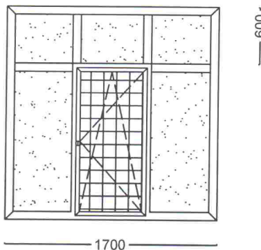
1. Ferestre parter,etajul N1; 1700-x2200(h) -24 buc
